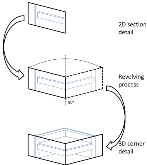
Fig. 1 – Conversion from 2D model to (revolved) 3D corner detail model
