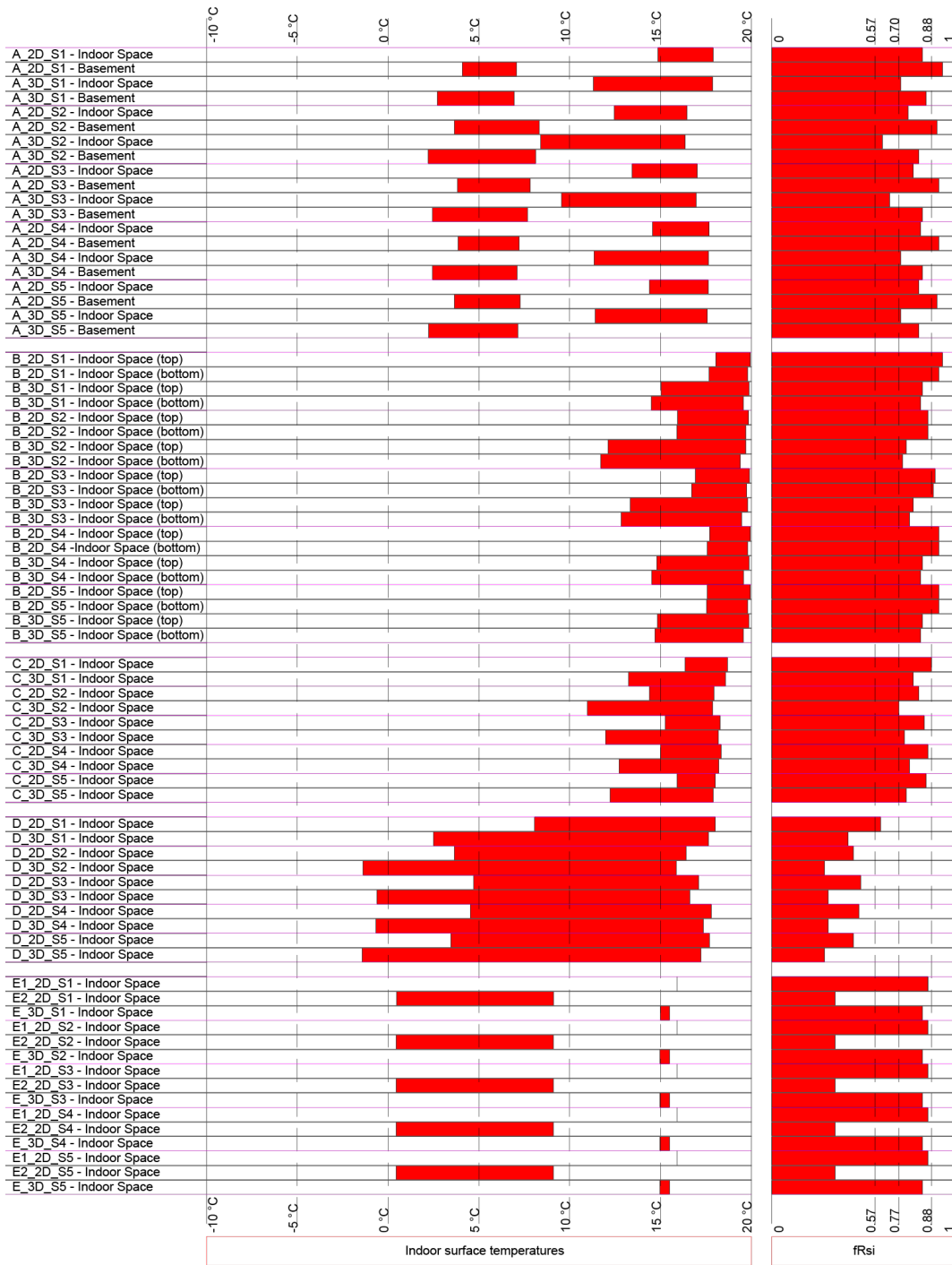
Fig 8 – Results overview (surface temperatures and f_{Rsi} values). Calculations are coded as {Detail_2D/3D-Simulation_Scenario}.
