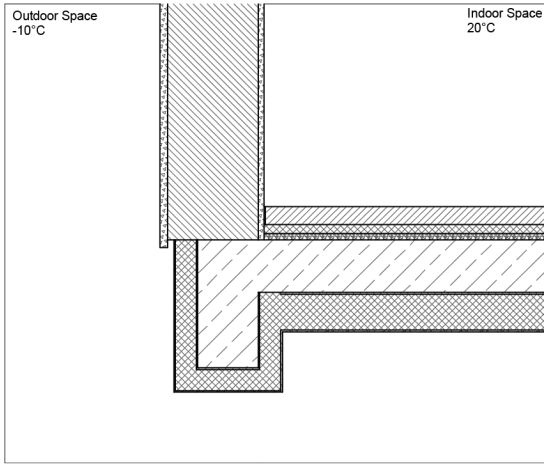
Fig. 6 - Detail D., Section 1:25
